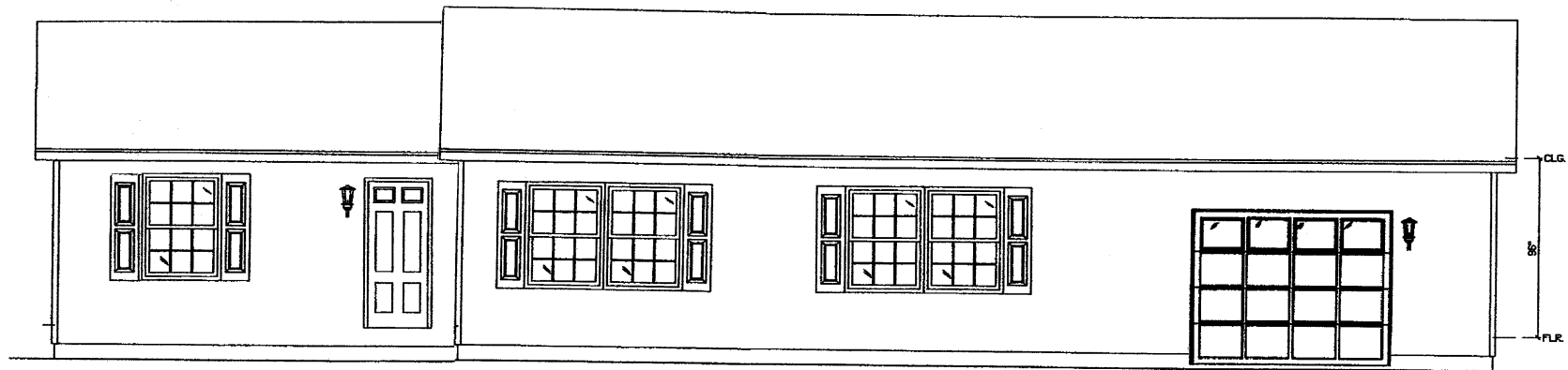
FRONT ELEVATION
