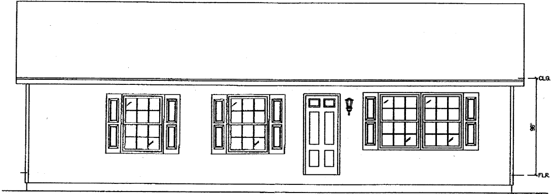
FRONT ELEVATION
